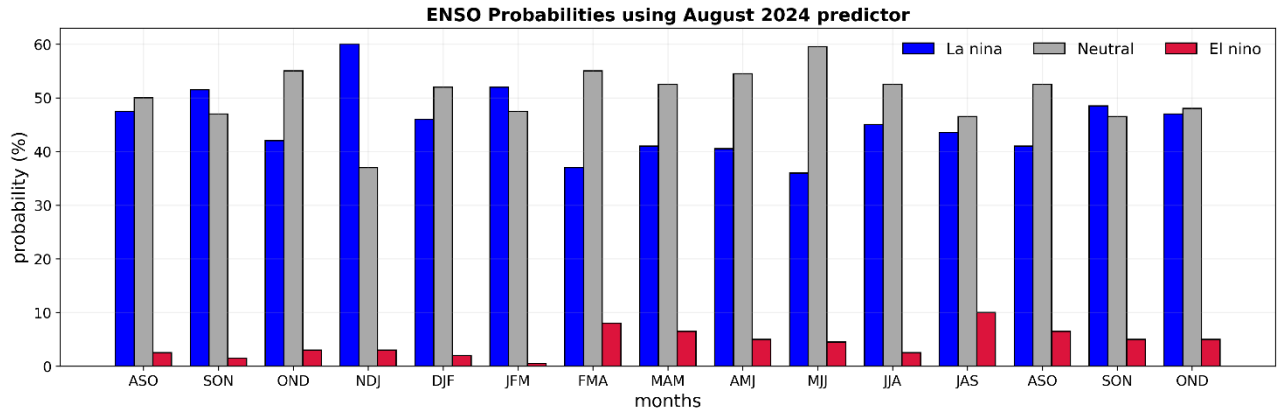
Fig. 5. Forecast of El Nino/La Nina conditions using June 2024-August 2024 predictors.
