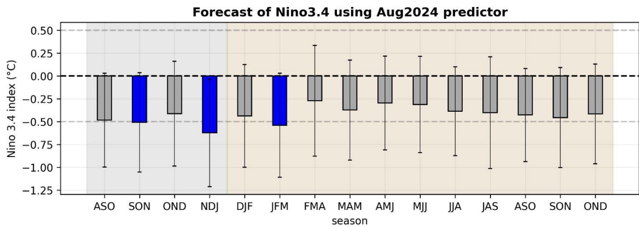
Fig. 4: Median prediction of Nino 3.4 index using June 2024-August 2024 predictors for the upcoming seasons.
