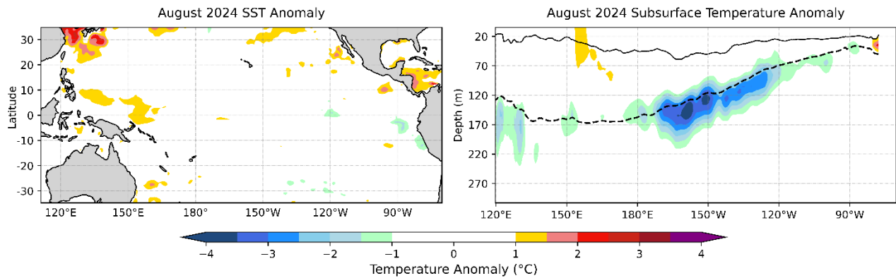
Fig. 3: (Left) Monthly SST anomaly for the tropical Pacific in August 2024. (Right) Subsurface temperature anomaly averaged over 5° S-5° N for August 2024.
