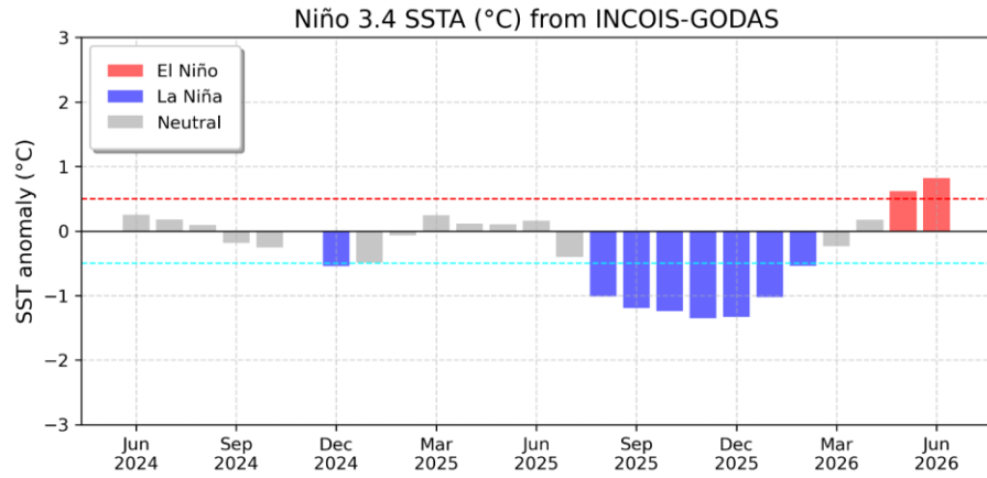
Fig. 1: Evolution of Sea Surface Temperature anomalies (°C) in the Niño 3.4 (5°S-5°N, 170°W-120°W) region in the period June 2024 - June 2026. The RED and CYAN horizontal lines represent 0.5°C SST anomaly
