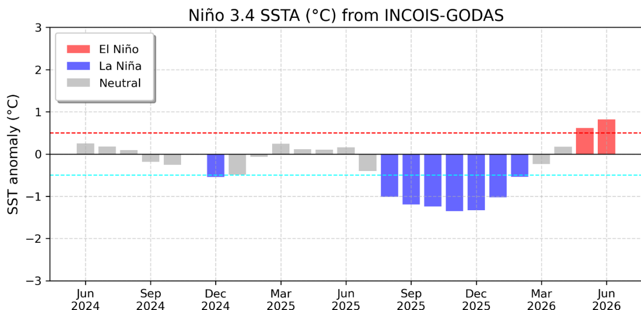
Fig. 1: Evolution of Sea Surface Temperature anomalies ( ^{\circ}\text{C} ) in the Niño 3.4 ( 5^{\circ}\text{S} - 5^{\circ}\text{N} , 170^{\circ}\text{W} - 120^{\circ}\text{W} ) region in the period June 2024 - June 2026. The RED and CYAN horizontal lines represent 0.5^{\circ}\text{C} SST anomaly
